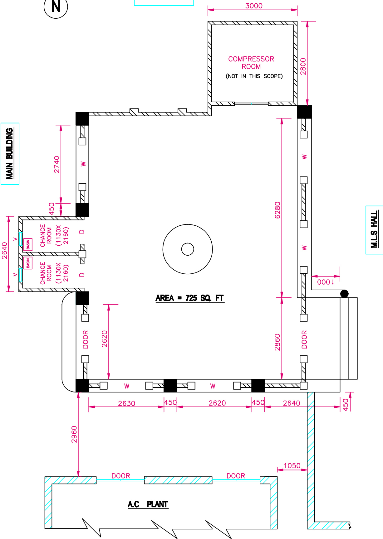
PLAN OF GYMNASIUM
