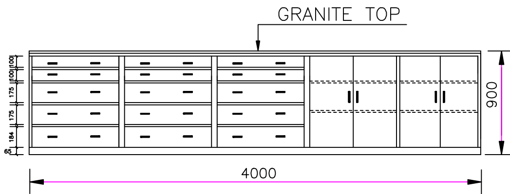
FRONT VIEW OF WORKING BENCH-2 (WOODEN)
