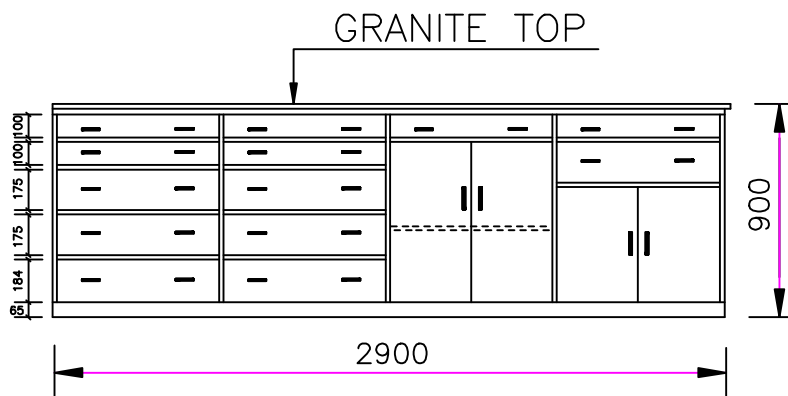
FRONT VIEW OF WORKING BENCH-1 (WOODEN)
