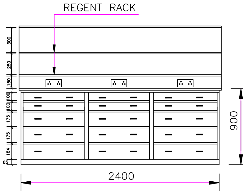
FRONT VIEW OF ISLAND BENCH FROM BOTH SIDE (WOODEN)
