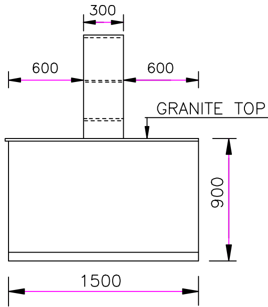
SIDE VIEW OF ISLAND BENCH
